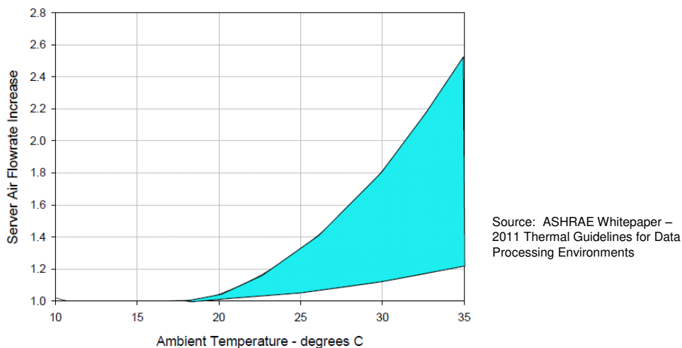
Figure 4. Relative change in server airflow with inlet temperature
